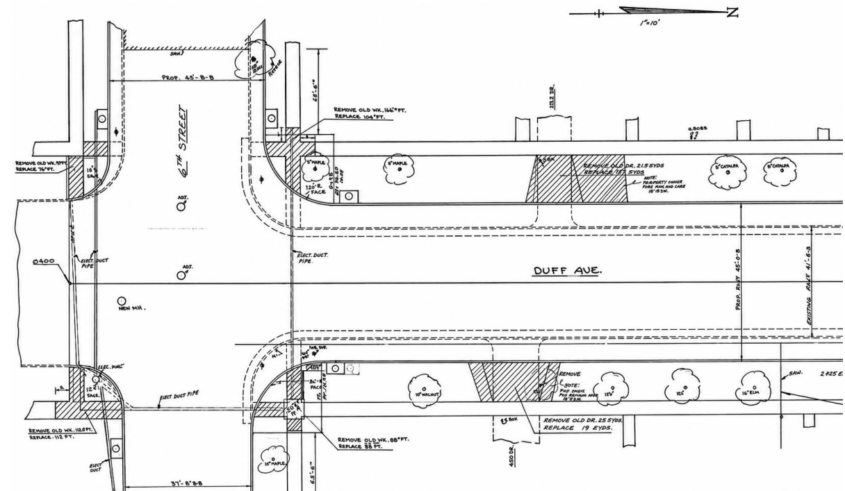
Duff Avenue 4-Lane Widening Project Plans (1962)
