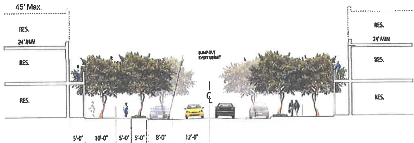
Figure 62: MLK JR. Blvd. Street Section
