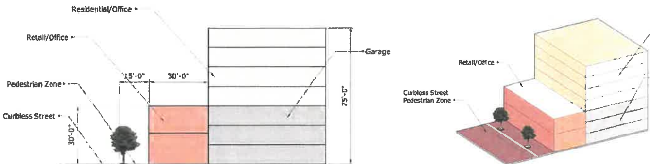
Figure 36: Ocean Ave. Design Diagram
