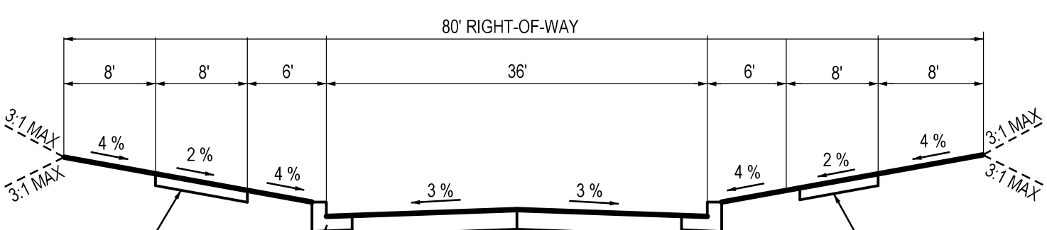
TYPICAL 80' RW CROSS SECTION
