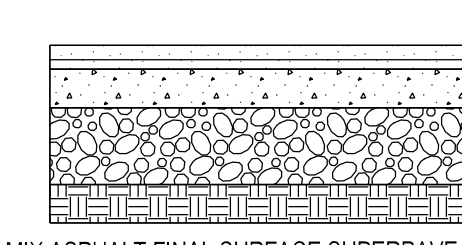
STANDARD PAVING SECTION P-3
