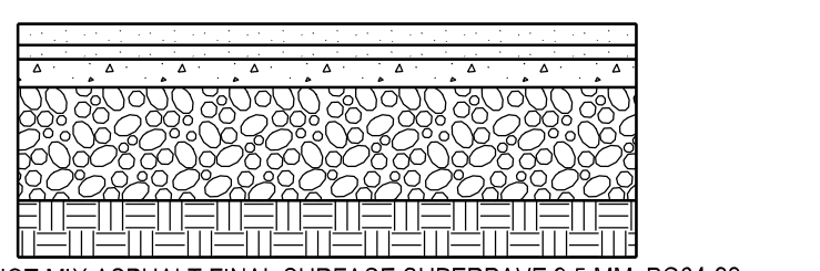
STANDARD PAVING SECTION P-2
