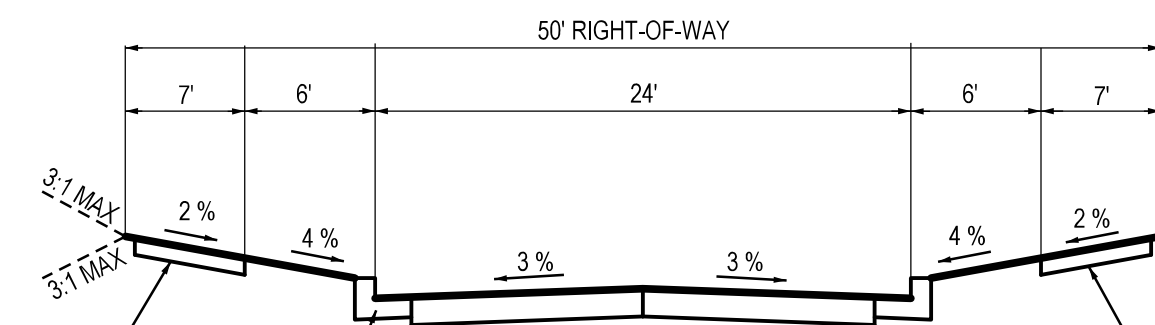
TYPICAL 50' RW CROSS SECTION
