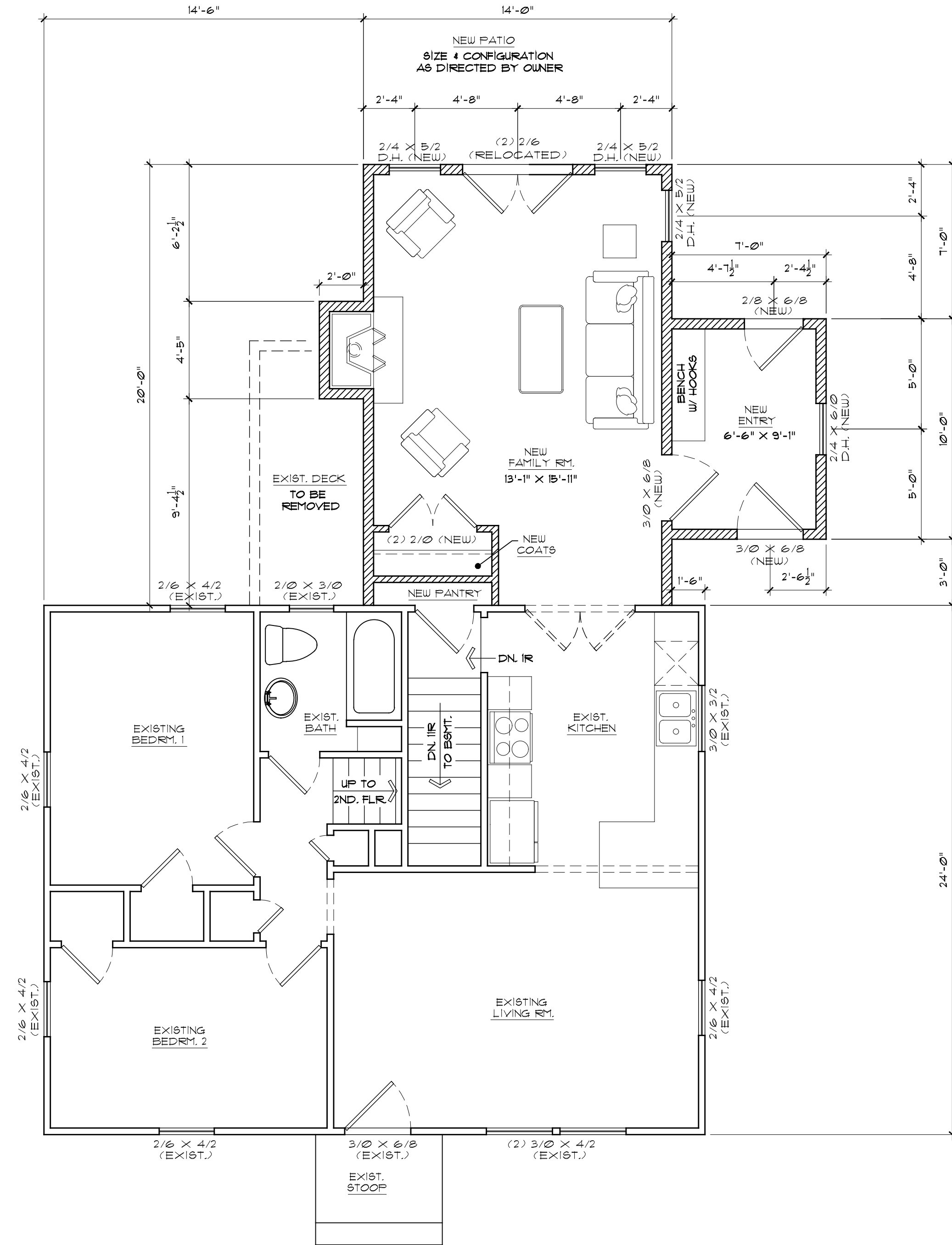
5 Preliminary Floor Plan P-1 Scale: 1/4" = 1'-0"
