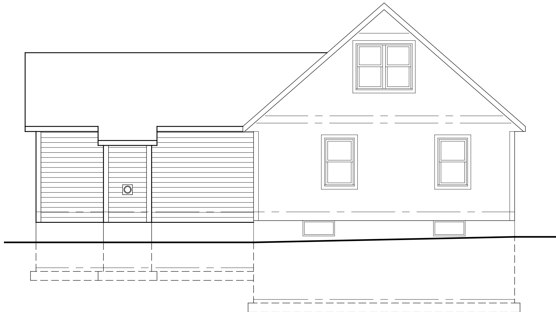
3 Preliminary Left Side Elevation P-1 Scale: 3/16" = 1'-0"
