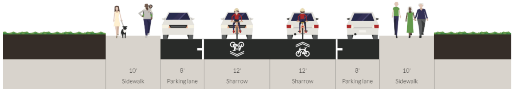
Arterial with On-Street Parking (60-foot ROW, 40-foot Paved Width)
