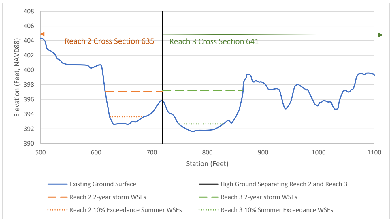
Figure 6: Basic Cross Section Schematic for Reach 2 and Reach 3 High Ground Split
