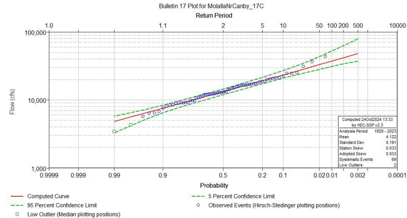
Figure 2: Bulletin 17C Plot for Molalla at Canby USGS Gage
