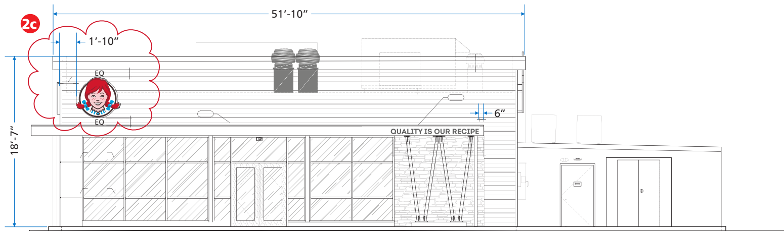
SOUTH ELEVATION SCALE 3/32" = 1'-0"
