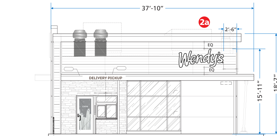
WEST ELEVATION SCALE 3/32"=1'-0"
