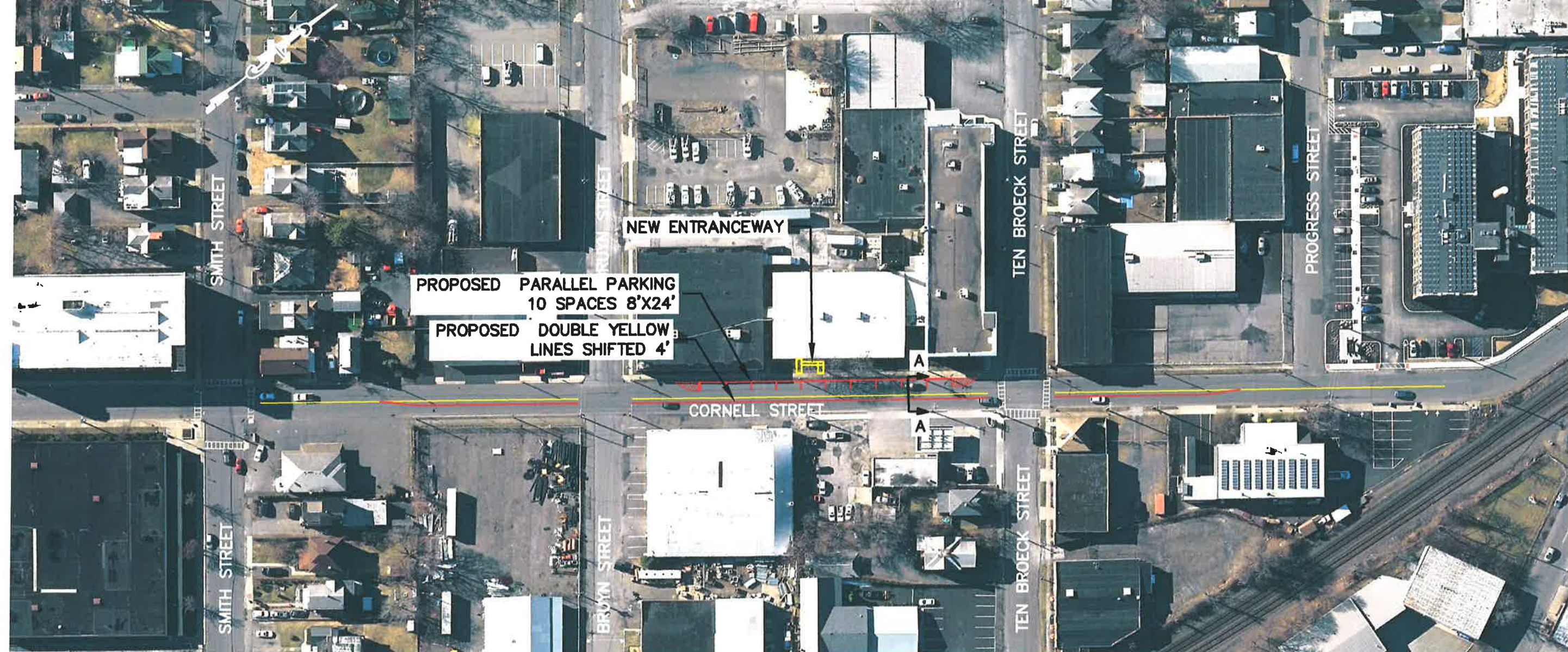
CONCEPT PLAN SCALE: 1" = 100'
