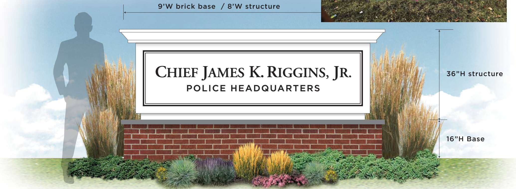
9'W x 16"H x 2'D - brick base with bluestone cap. 1/4" thick painted aluminum lettering - 6"H and 4"H Aluminum sign cabinet structure with decorative Fypon Applied mouldings.
