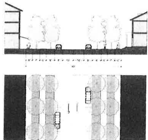
Typical Street Section
