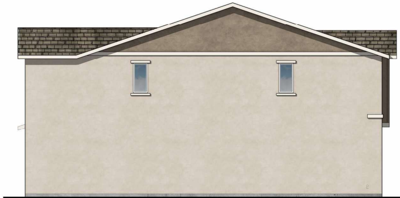
LEFT ELEVATION ELEVATION A 1/4" = 1'-0"
