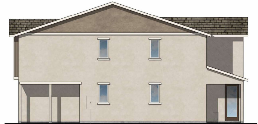
RIGHT ELEVATION ELEVATION A 1/4" = 1'-0"
