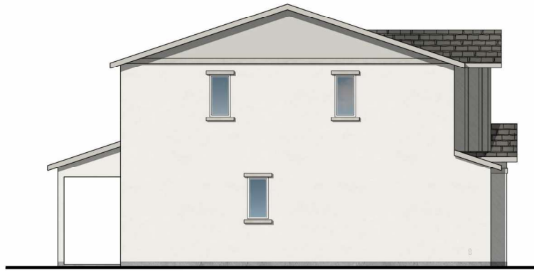
LEFT ELEVATION ELEVATION A 1/4" = 1'-0"
