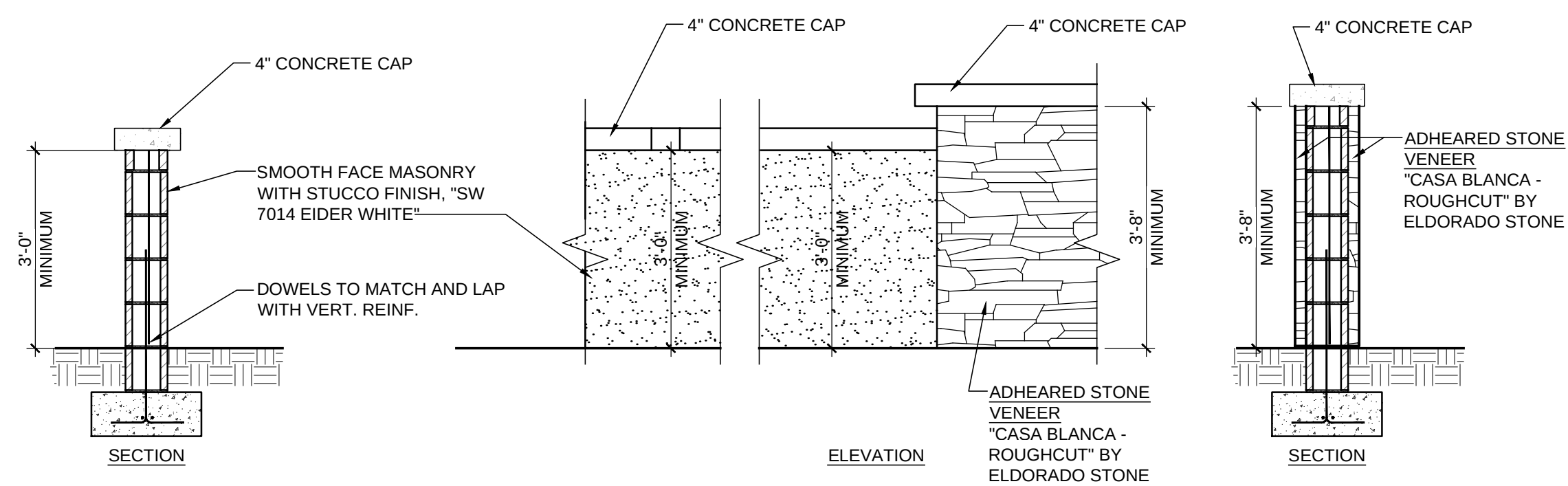
5 SITE SCREEN WALL - SECTION / ELEVATION SCALE: 1/2" = 1'-0"
