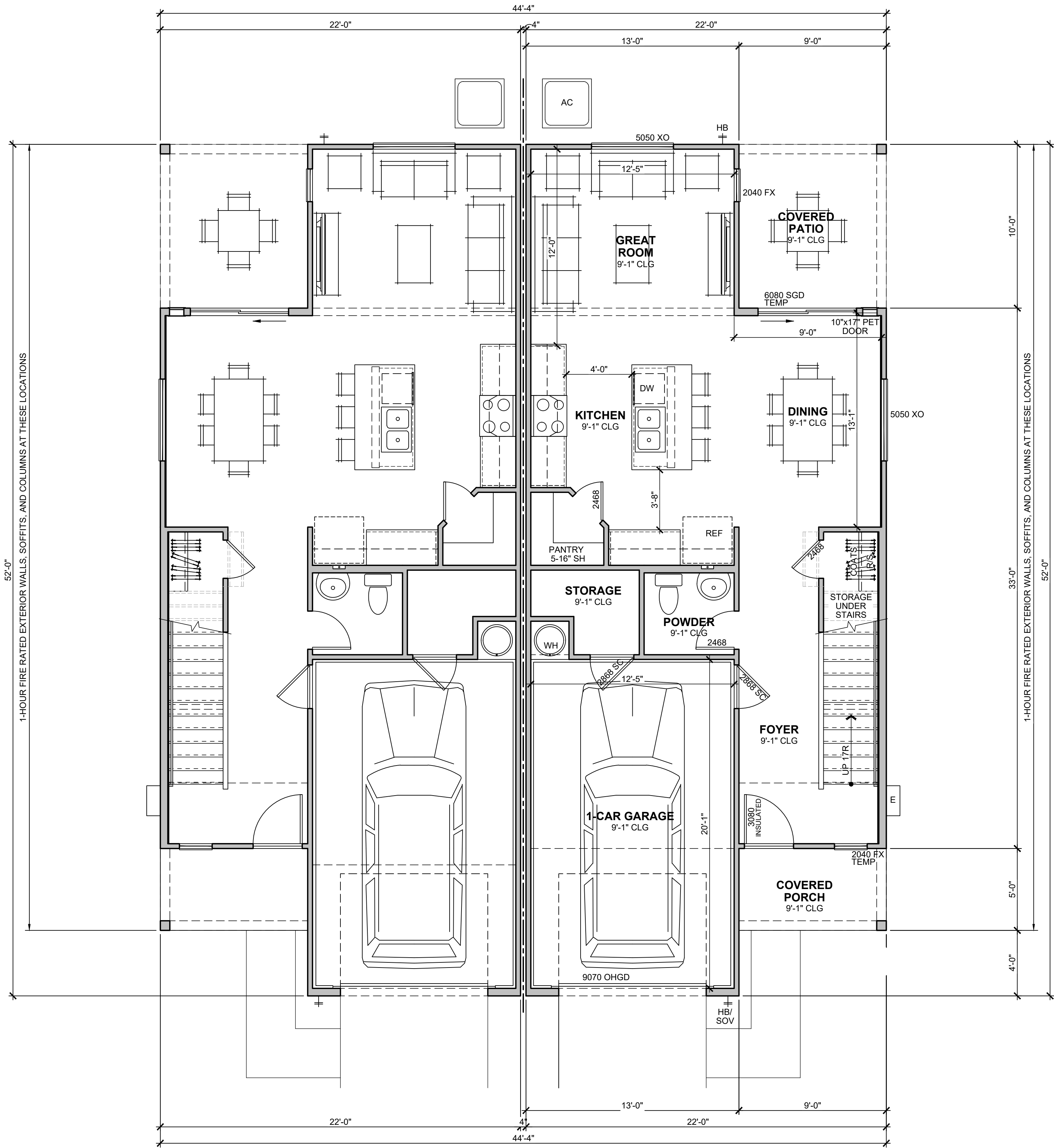
FIRST FLOOR PLAN 1/4" = 1'-0"
